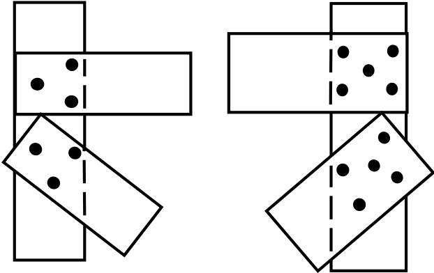
2x6 to POSTS
