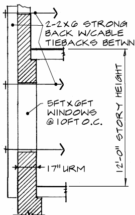
WINDOW SECTION
