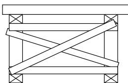
5ft to 8ft o.c. Bracing between Shores
