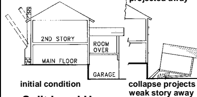
Split Level House
